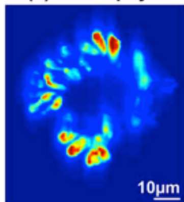
(b) Chlorophyll
