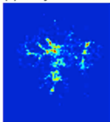
(e) Botryococcenes
