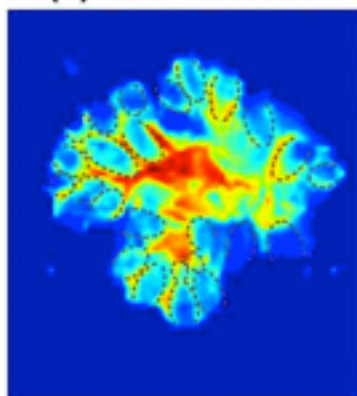
(c) Carotenoids
