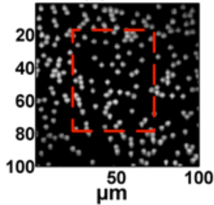
(c) PS
