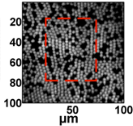
(b) PMMA
